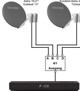
Beispiel 2: 4 Satelliten (Single-LNBs) Astra 19,2° Eutelsat 13° Eurobird-Astra 28,5° Türksat 42°
