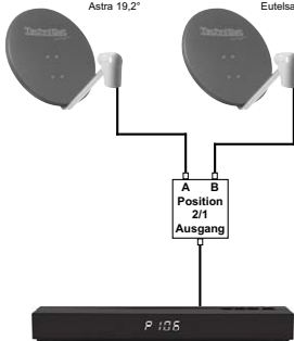
Beispiel 1: 2 Satelliten (Single-LNBs) Astra 19,2° Eutelsat 13°
